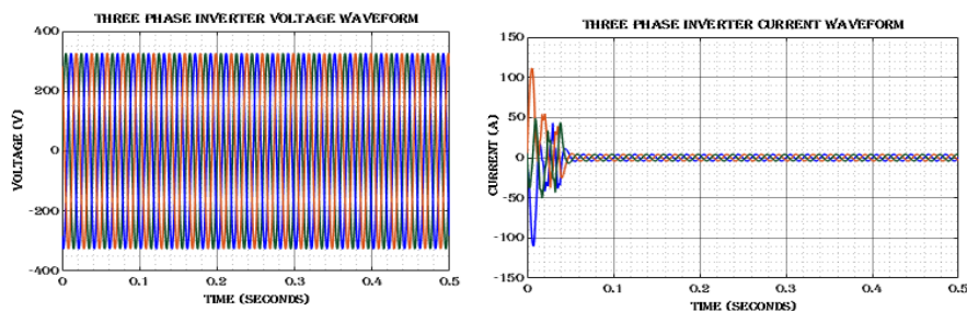
Figure 11: Inverter Waveform
