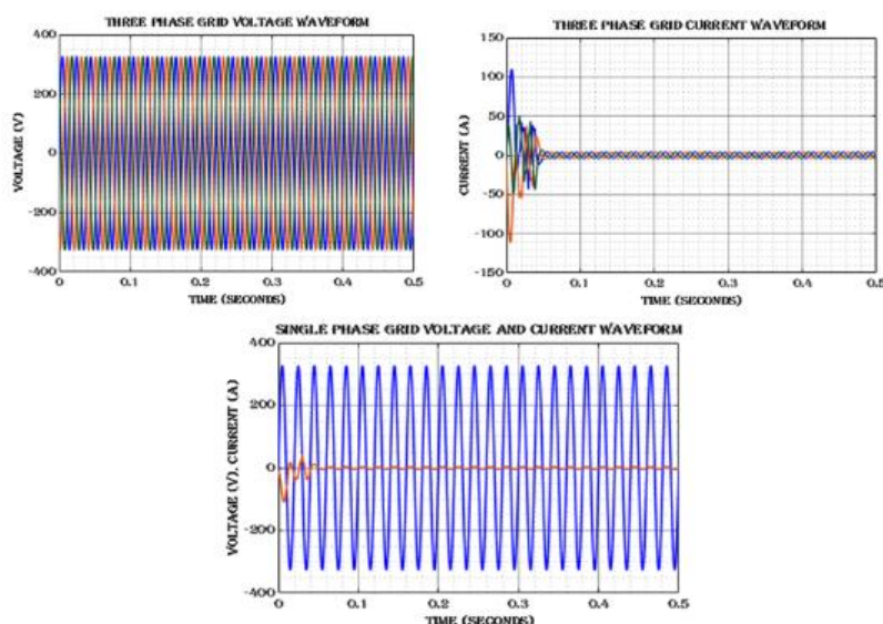
Figure 12: Grid Voltage Waveform
