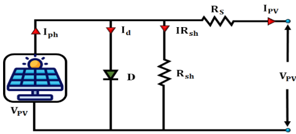
Figure 2: Equivalent model of solar cell
