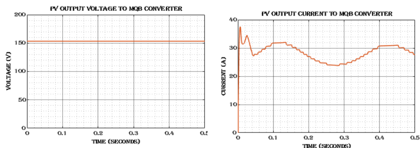
Figure 8: Converter Output Waveform
