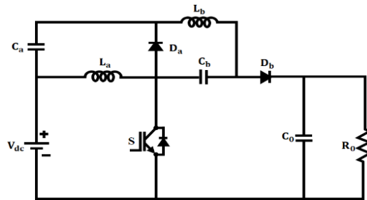
Figure 3: Circuit Diagram of MQBC
