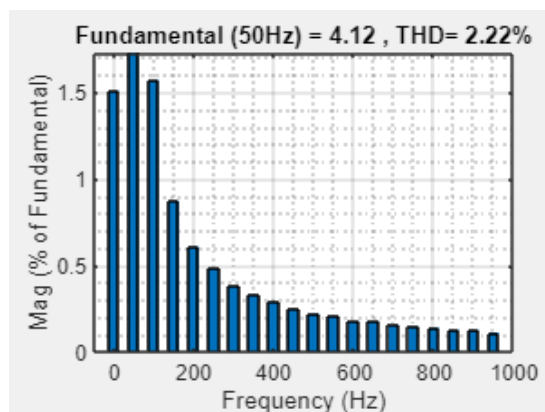
Figure 13: THD Waveform
