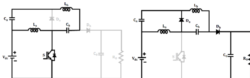
Figure 4: Modes of Operation
