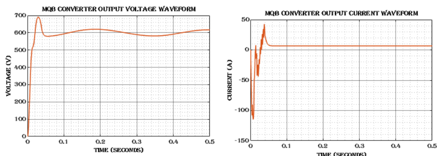
Figure 9: Converter Output Waveform
