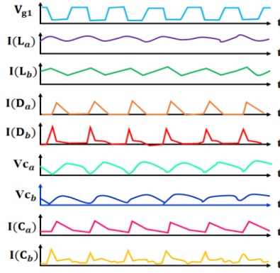
Figure 5: Operating Waveform
