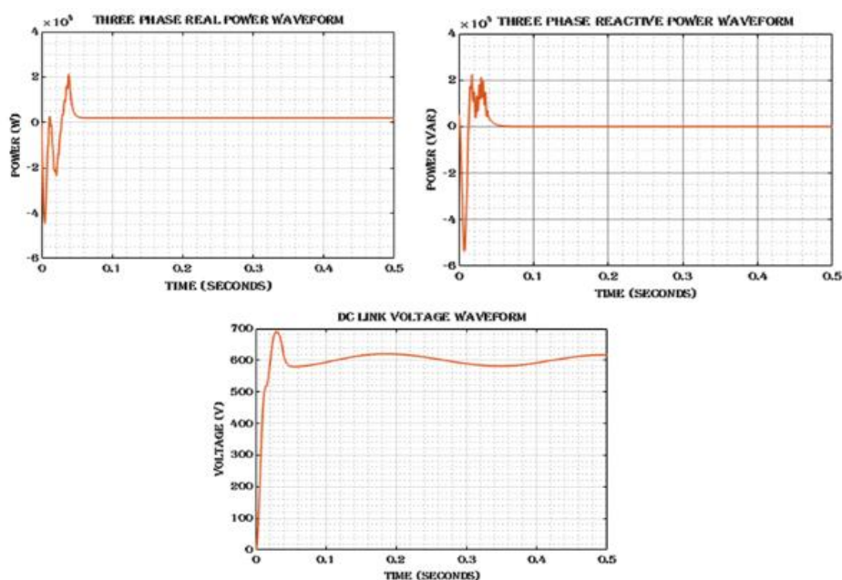
Figure 10: Power and Voltage Waveform
