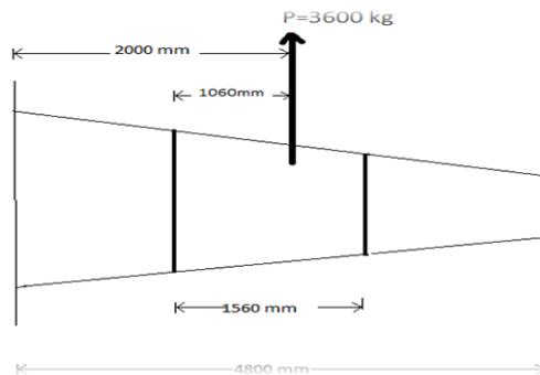
Figure 2(b): Wing box dimensions with load.
