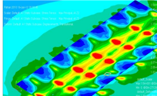
Figure 3(d): maximum stress at rivet holes of the splice plate
