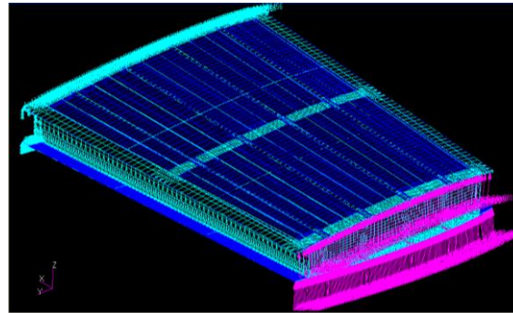
Figure 3(a): wing box loading conditions
