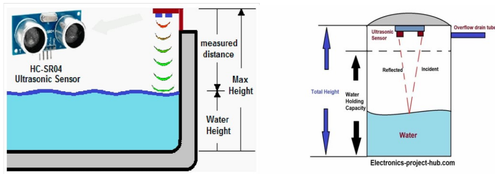
Figure 2: Schematic of Water Level monitoring process
