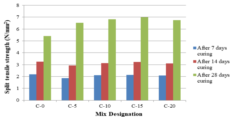
Chart 2: Variation in split tensile strength
