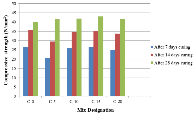
Chart-1: Variation in compressive strength
