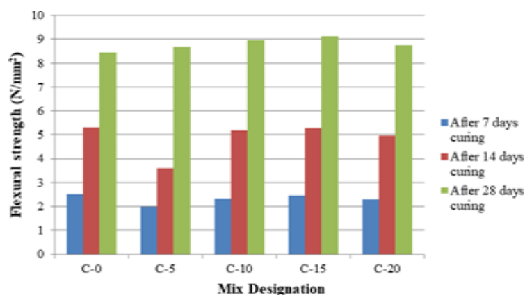
Chart 2: Variation in flexural strength
