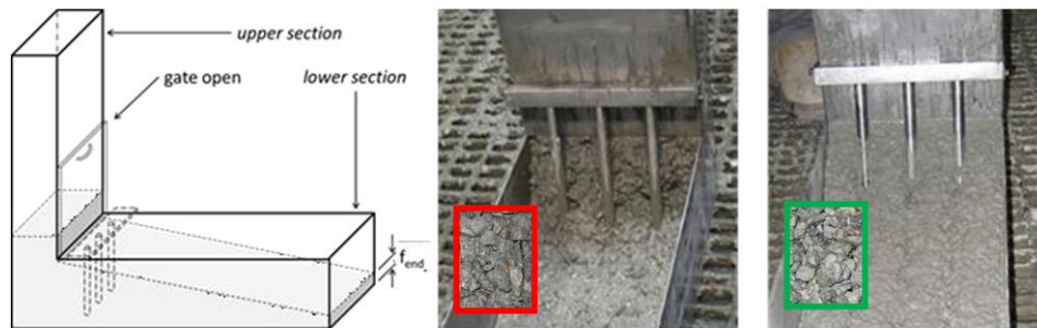
Figure 8: Schematics of the L-box test (left), effects of the aggregate shape on the passing-ability of a highly flow-able tremie mix (centre, right)
