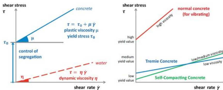
Figure 7: Rheological behaviour of concrete in general (left) and for different concrete types (right), after EFFC/DFI Best Practice Guide to Tremie Concrete for Deep Foundations, 2016
