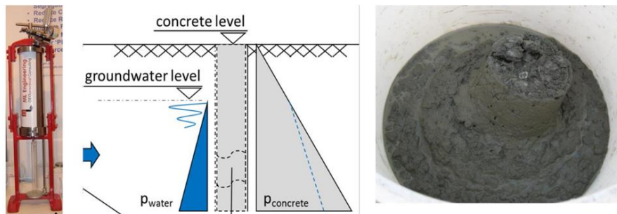
Figure 9: The filtration test apparatus (left) helps to detect tendencies of concrete bleeding under pressure in fresh concrete (centre) which results in changes in rheology, effecting flow
