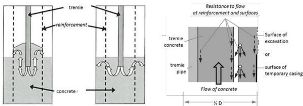
Figure 6: Risk of concrete rising faster inside the reinforcement causing fluid inclusions in the cover area (left) and schematics of 'resistance of concrete flow' during a tremie pour
