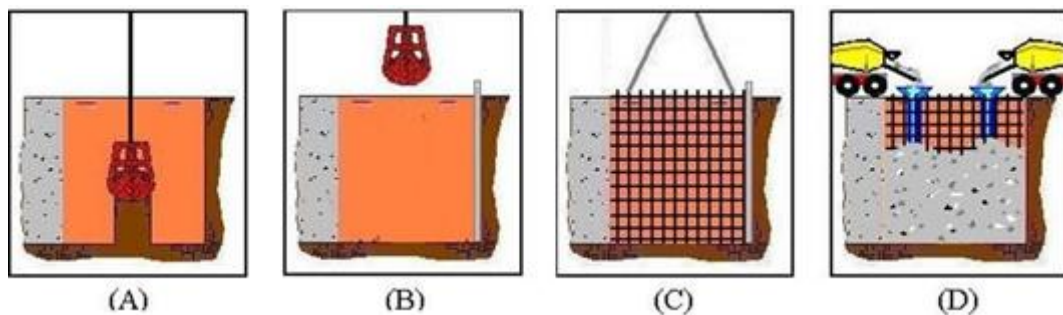
Figure 2: Typical construction sequence of a diaphragm wall panel–(A) panel excavation, Recycling /replacement of drilling fluid and placement of stop-end with water bar, (C) reinforcement cage installation and(D)concrete place mentusing the Tremie method
