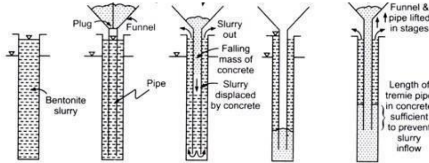
Figure 5: Typical tremie pour for a diaphragm wall panel installed under bentonite fluid
