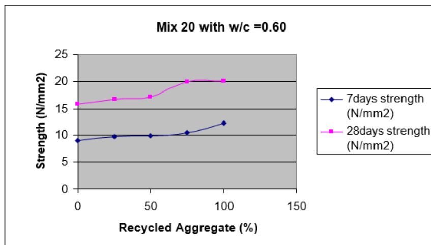
Figure 8: Compressivestrengthat7days&28daysofM20concrete with w/c=0.60
