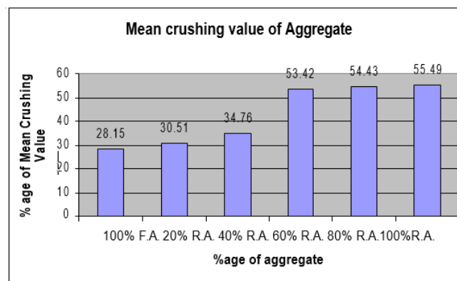
Figure 2: Mean crushing value of aggregate for different %age of R.A
