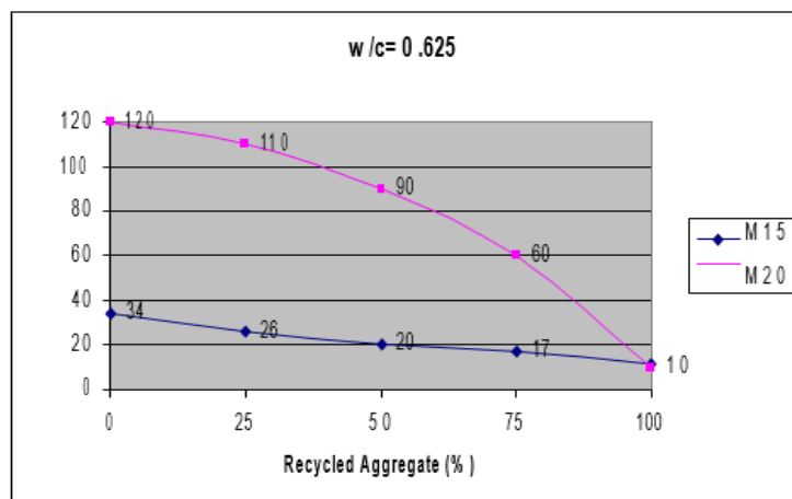
Figure 4: Slump value of M15 & M20 concrete with w/c=0.625
