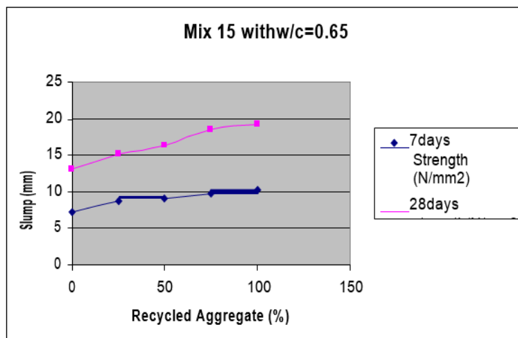
Figure 7: Compressivestrengthat7days&28daysofM15concrete withw/c=0.65
