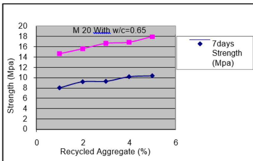
Figure 9: Compressivestrengthat7days&28daysofM20concrete withw/c=0.65
