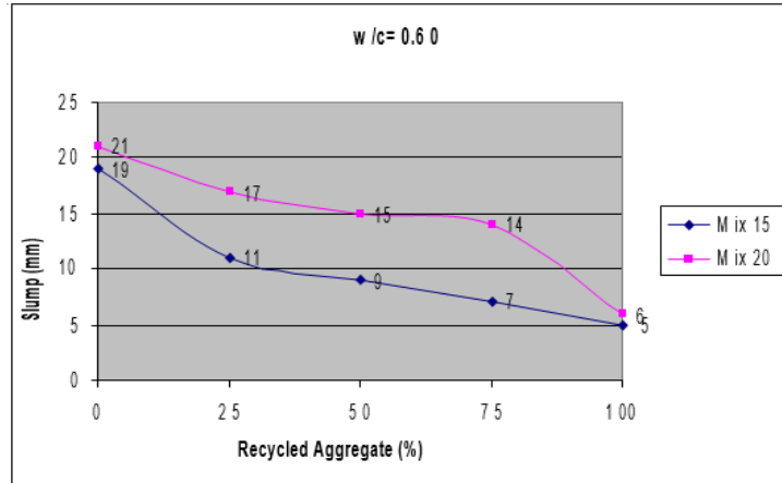
Figure 3: Slump value of M15 & M20 concrete with w/c=0.60
