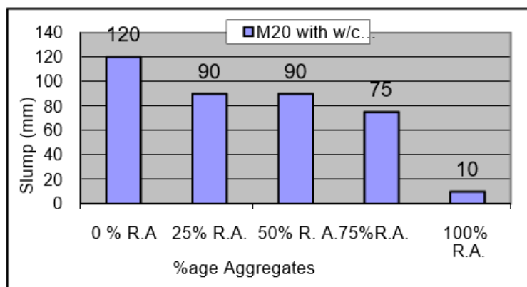
Figure 5: Slump value of M20 concrete with w/c = 0.650
