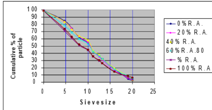
Figure 1: Average sieve analysis test of aggregate
