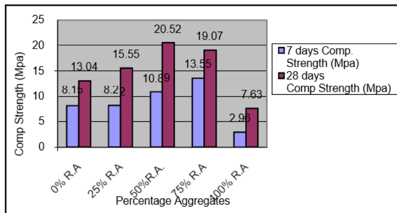
Figure 6: Compressivestrengthat7days&28daysofM15 concrete with w/c=0.60
