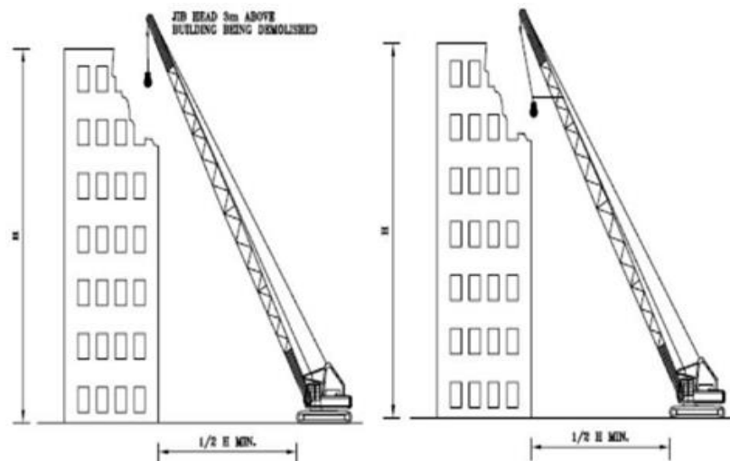
Figure 7: Operation using Wrecking Ball
