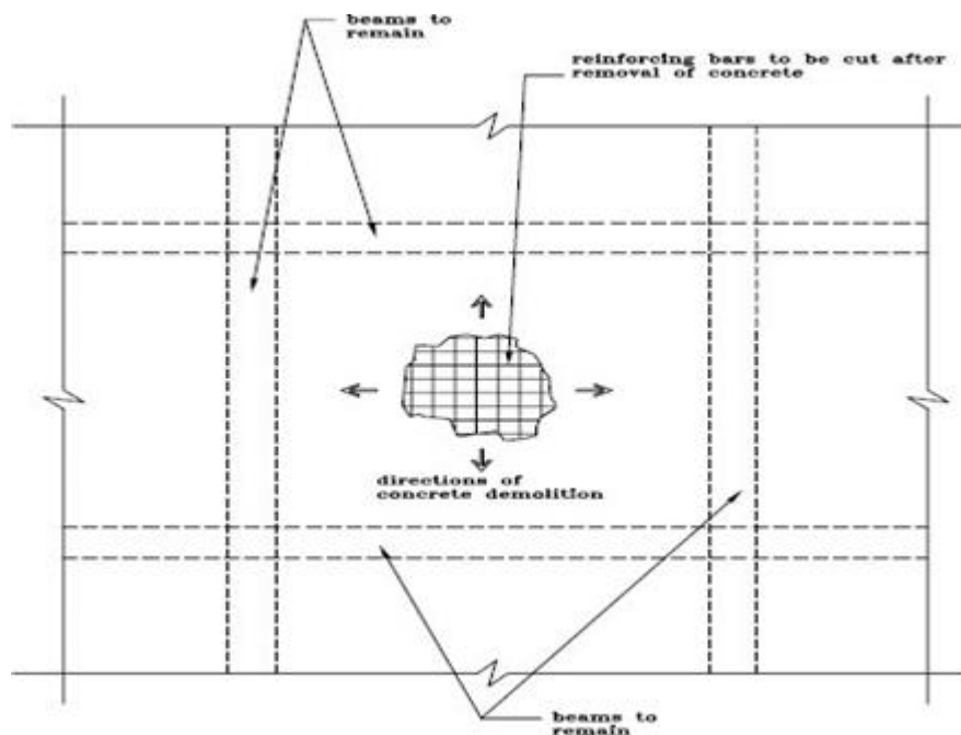
Figure 2: Demolition of slab
