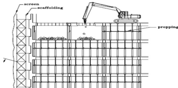
Figure 4: Continue Demolition of Slabs and Beams
