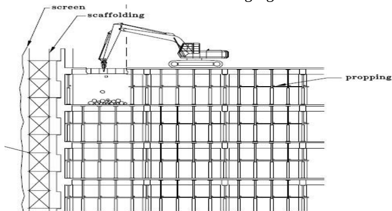
Figure 3: Demolition of Slabs and Beams
