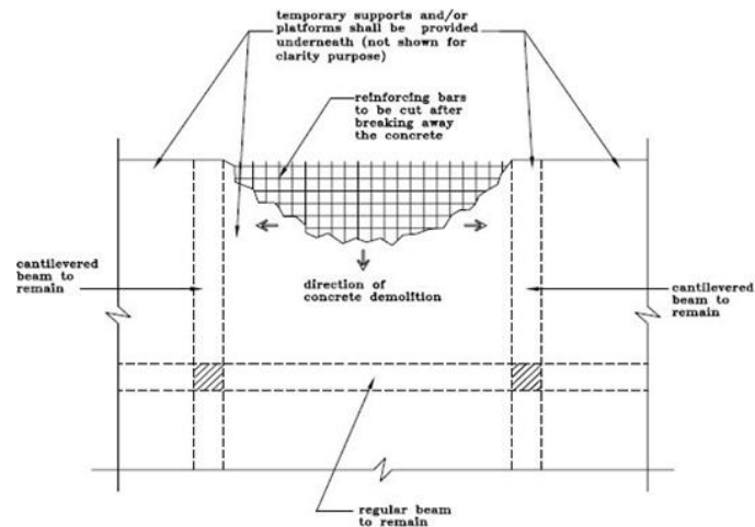
Figure 1: Demolition of cantilevered RCC slab (Manual method)
