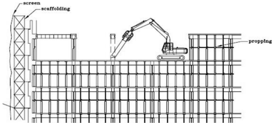
Figure 6: Demolition of interior column
